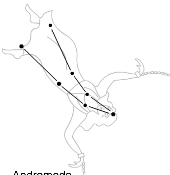
Andromeda
